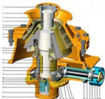
Vertical crusher
